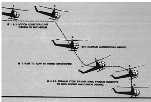
FIGURE 77—Flare autorotation and touchdown.
